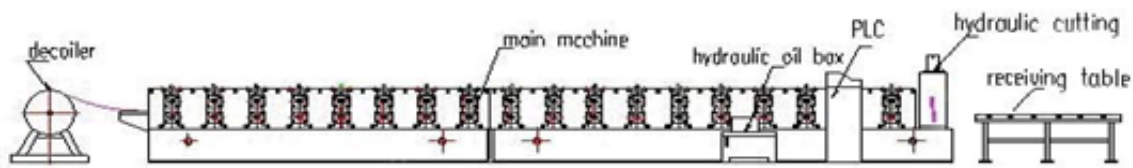
Deck Floor Roof Sheet Roll Forming Machine details
